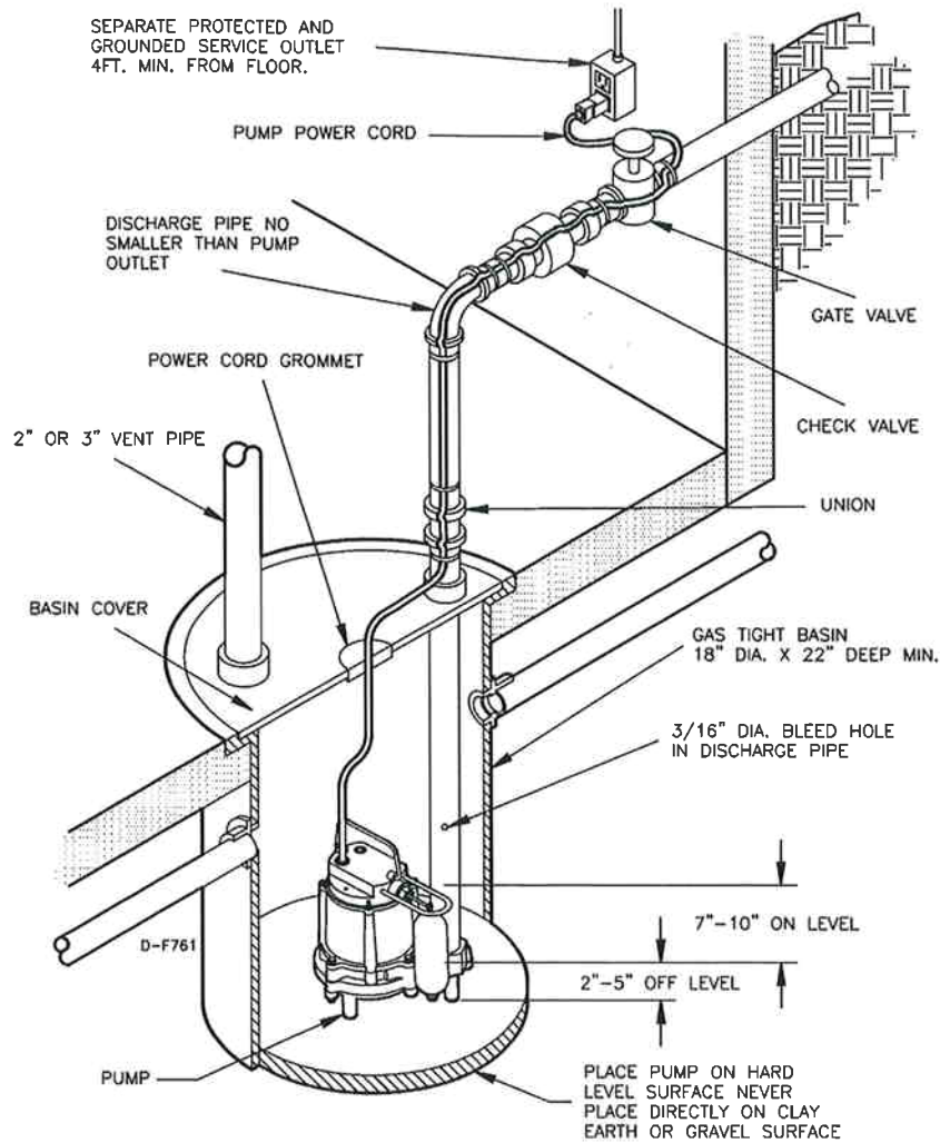
Figure 1. Typical Installation
